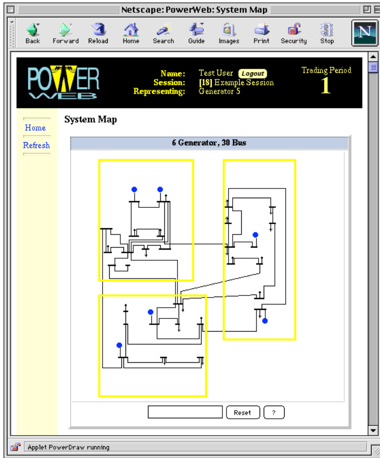
Figure 3: PowerWeb one-line diagram display, showing 30-bus system
